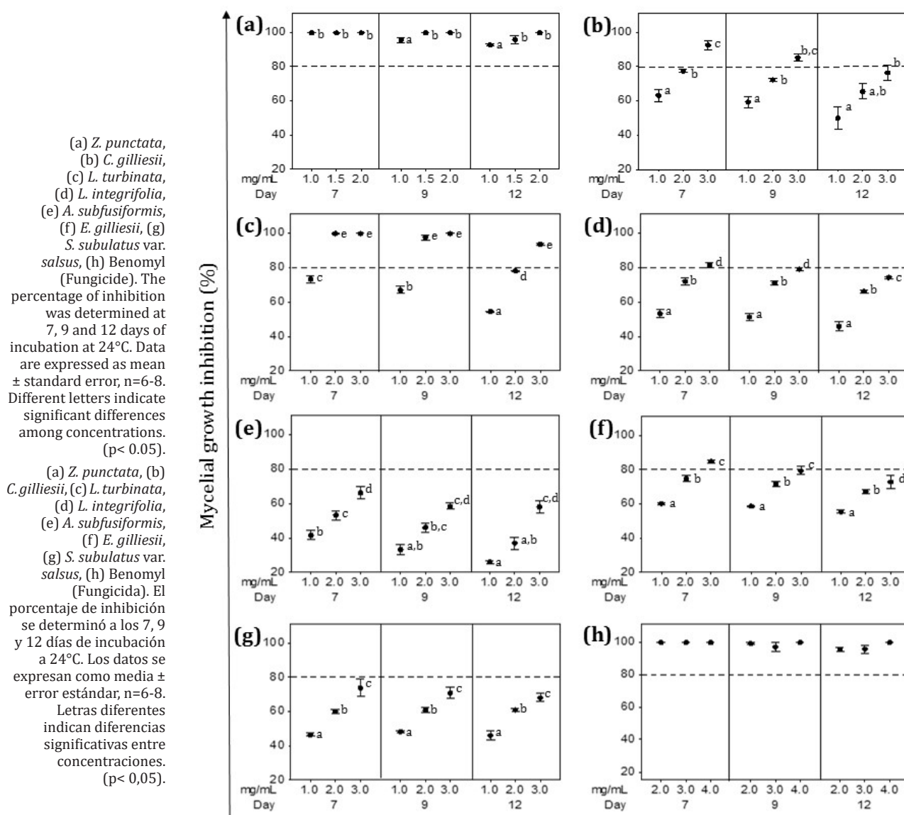
Figure 5. Effect of ethanolic extracts (EEs) on P. parasiticum mycelial growth.
