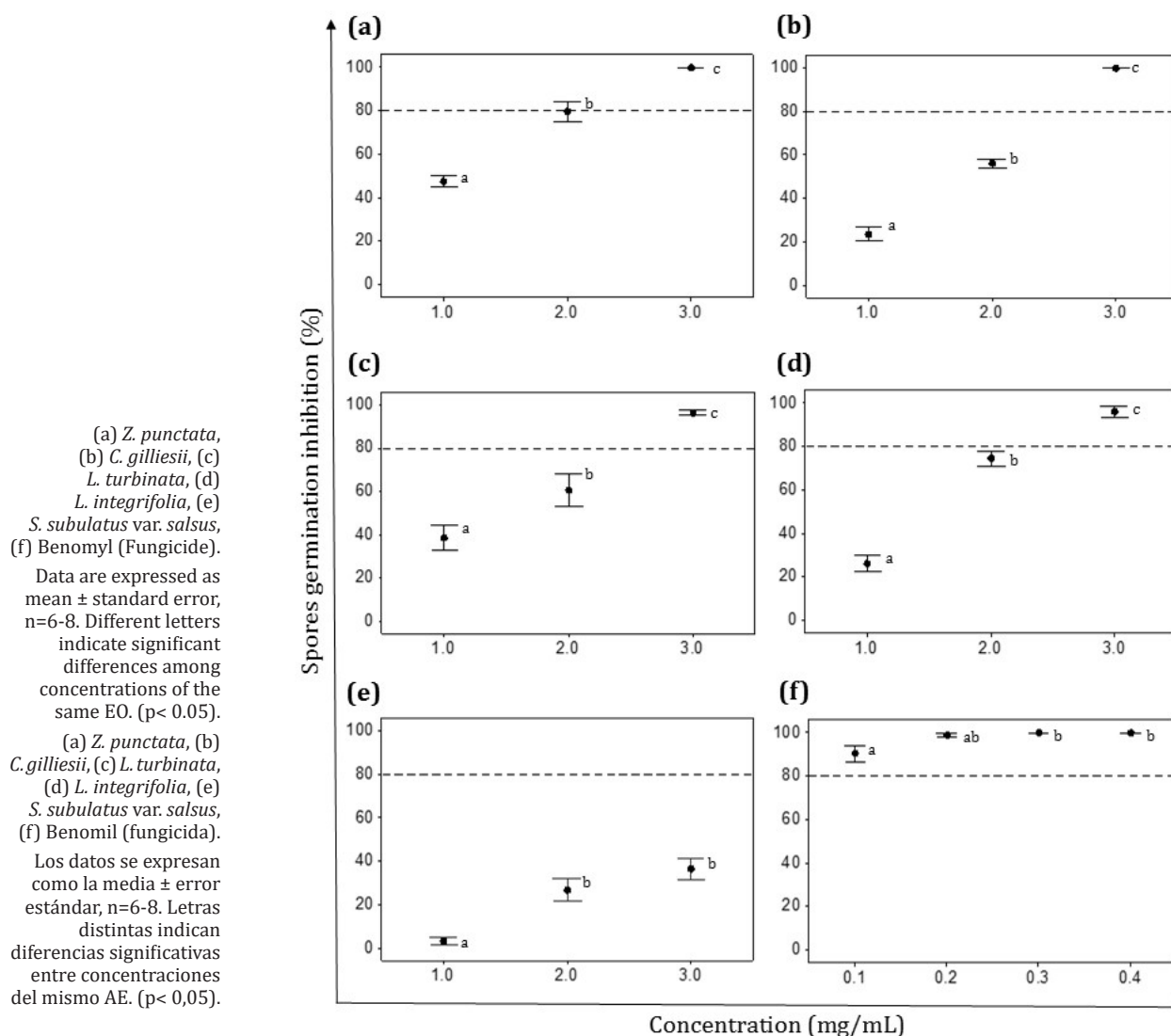
Figure 1. Effect of essential oils (EOs) on V. dahliae spore germination.
