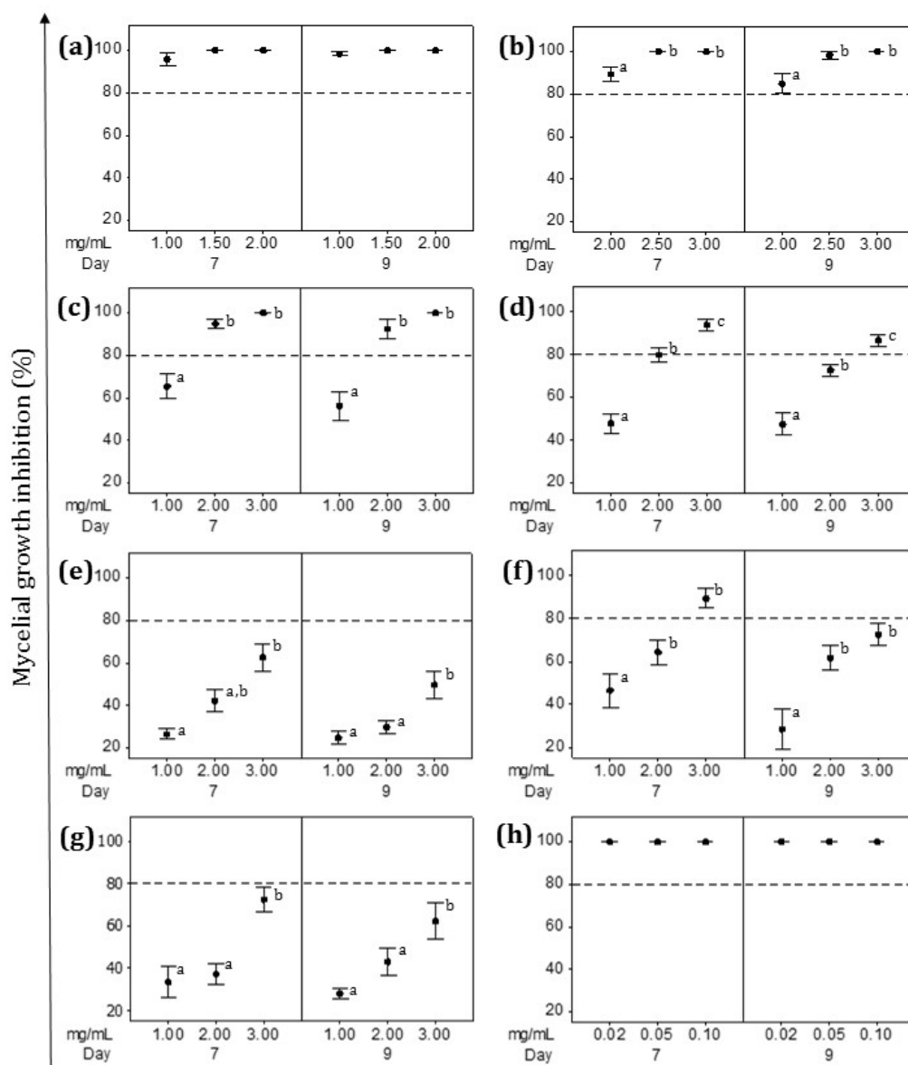
Figure 4. Effect of ethanolic extracts (EEs) on V. dahliae mycelial growth.
